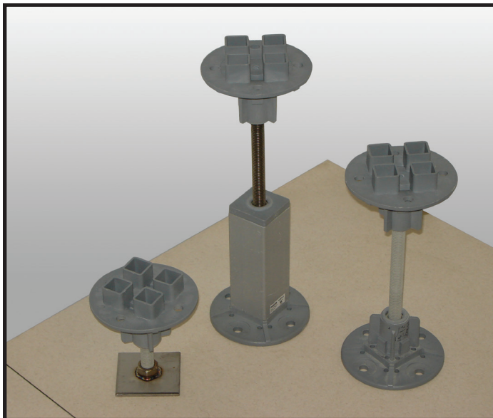
*Pedestals as short as 3.5" are available on request. Contact Fibergrate for details.
