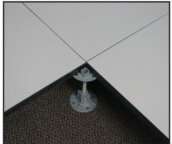
Fibergrate's Quad Head pedestals can be located anywhere within the Micro-Mesh® panel or to join two or four panels as shown.
